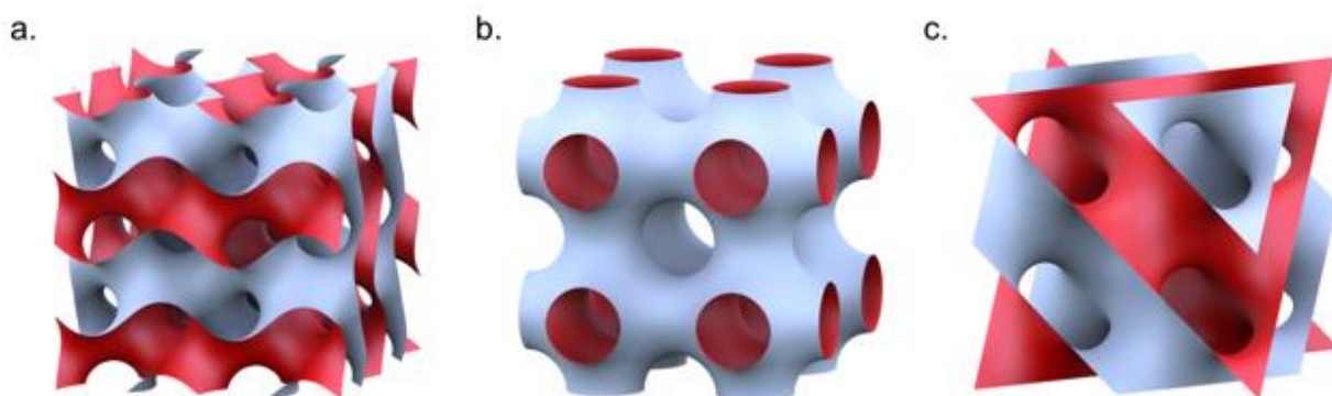
Figure 2. Examples of three triply periodic minimal surfaces. a. Gyroid b. Primitive cubic surface and c. Diamond cubic surface. Adapted from [16] Copyright 2014, Walter de Gruyter Berlin/Boston
