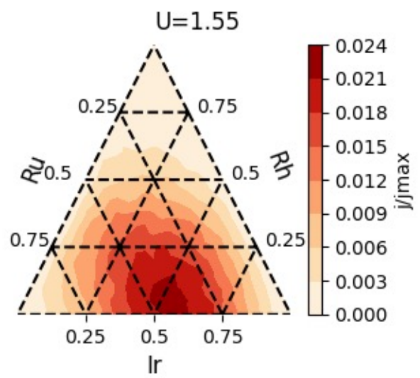
Composition-dependent current
